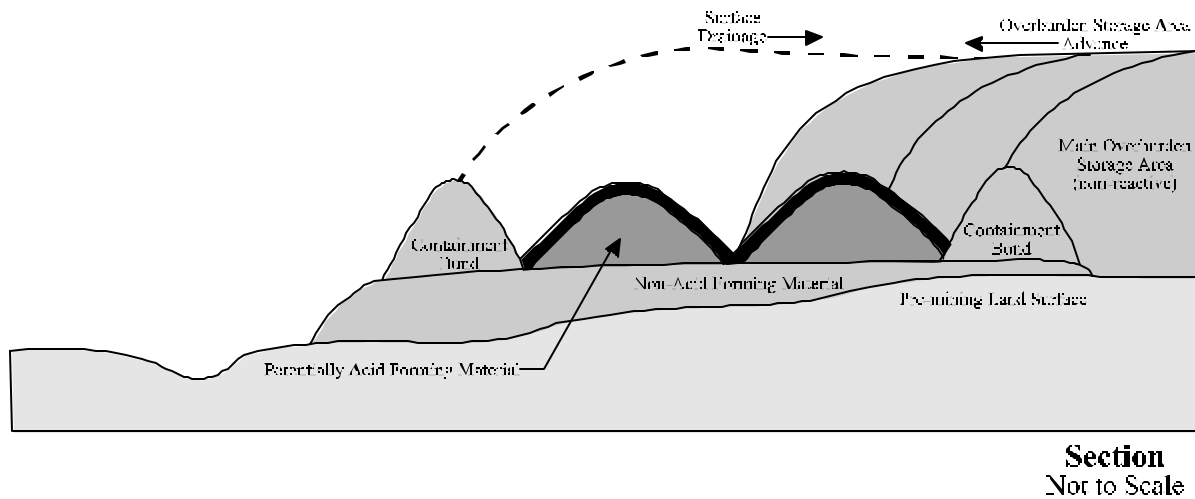
Figure 1 Schematic representation of encapsulation method for potentially acid forming waste rock.
