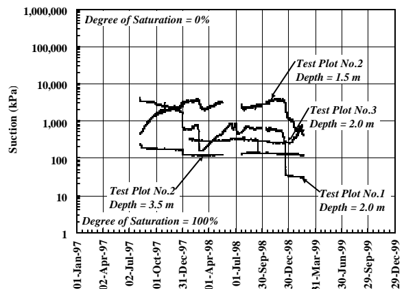
Figure 4 Depth of infiltration measured by soil suction sensor response in Test Plot No.1 (2.0 m), Test Plot No.2 (1.5 m and 3.5 m), and Test Plot No.3 (2.0 m).
