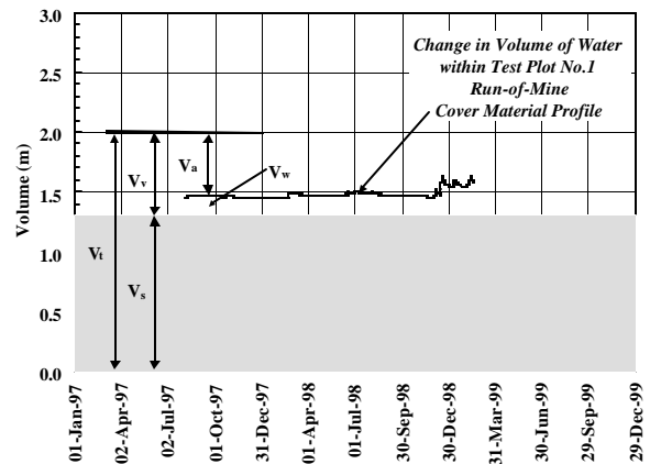
Figure 2 Cumulative change in moisture storage (i.e. V_w ) in Test Plot No.1 run-of-mine cover material profile.
