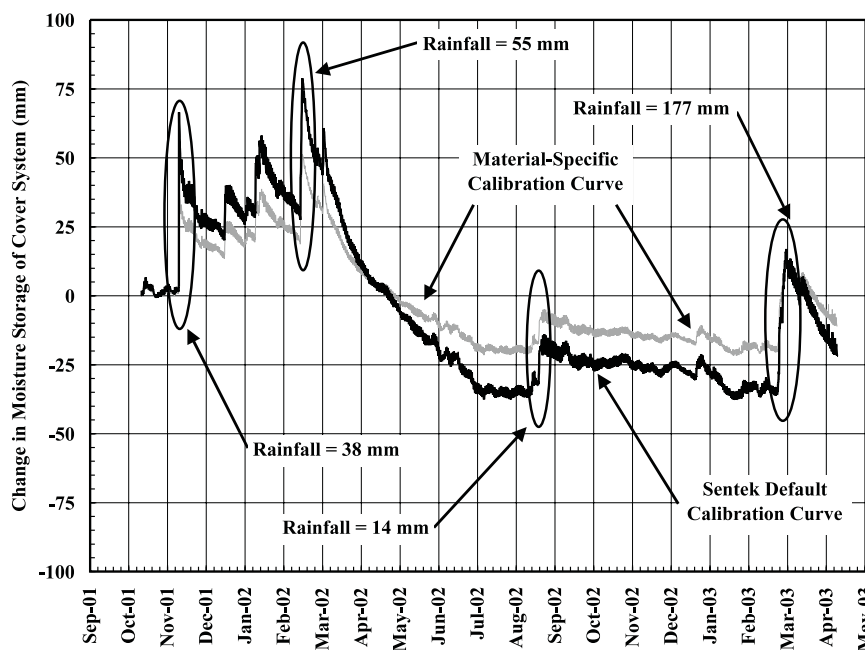
FIG 4 - Change in moisture storage within the tailings storage facility cover system measured with EnviroSCAN® sensors.
