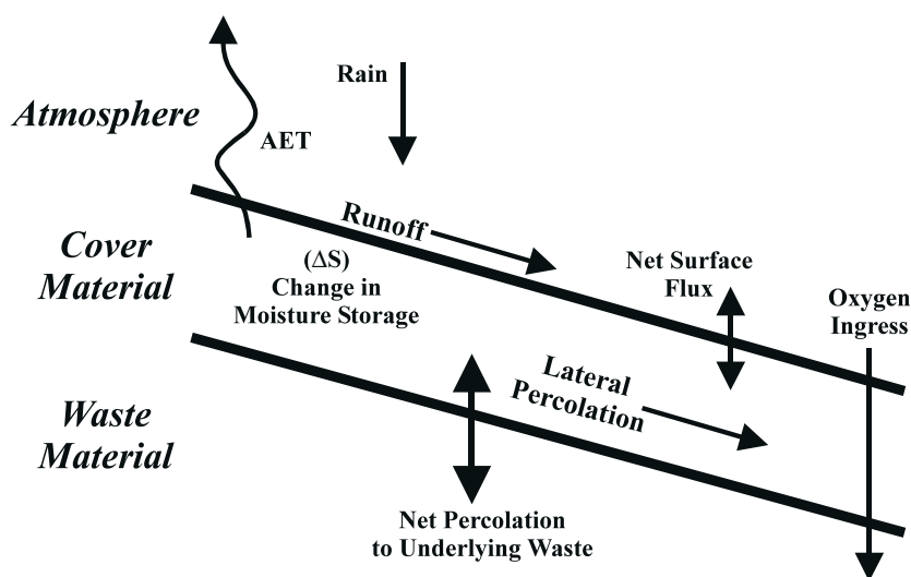
FIG 1 - Components of water balance calculation for dry cover systems.
