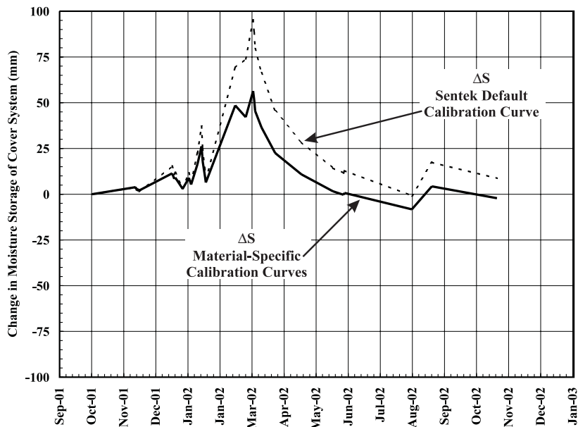
FIG 5 - Change in moisture storage within the tailings storage facility cover system measured with Diviner 2000® sensor.
