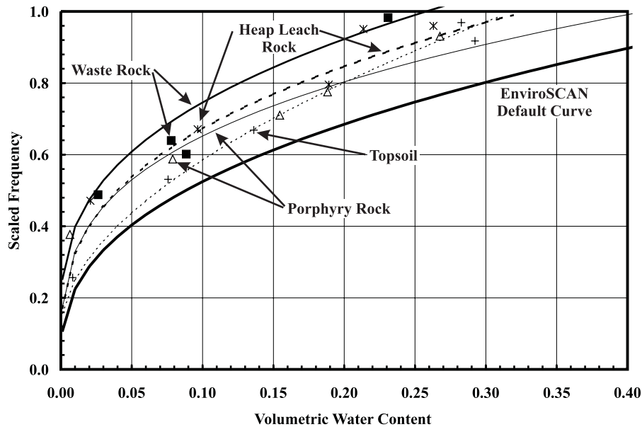
FIG 3 - Sample of the laboratory calibration results for the EnviroSCAN® sensor.
