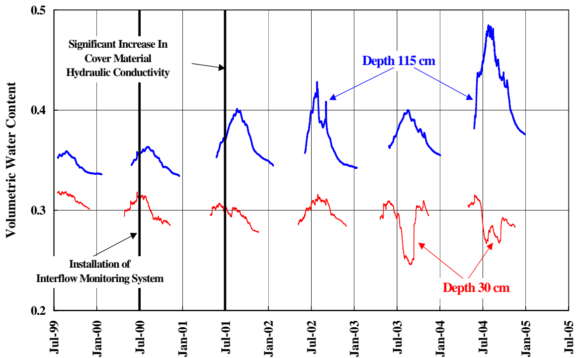
Figure 5. Monitored volumetric water contents within the 100 cm cover.
